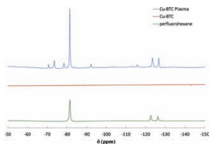
Figure 2. ^{19}\text{F} MAS NMR of Cu-BTC plasma, Cu-BTC, and neat PFH. All spectra are referenced to an external hexafluorobenzene reference \delta \approx -165 ppm.
