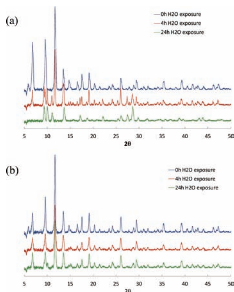
Figure 1. PXRD patterns for (a) Cu-BTC and (b) Cu-BTC plasma after immersion in water at room temperature for 0, 4, and 24 h.
